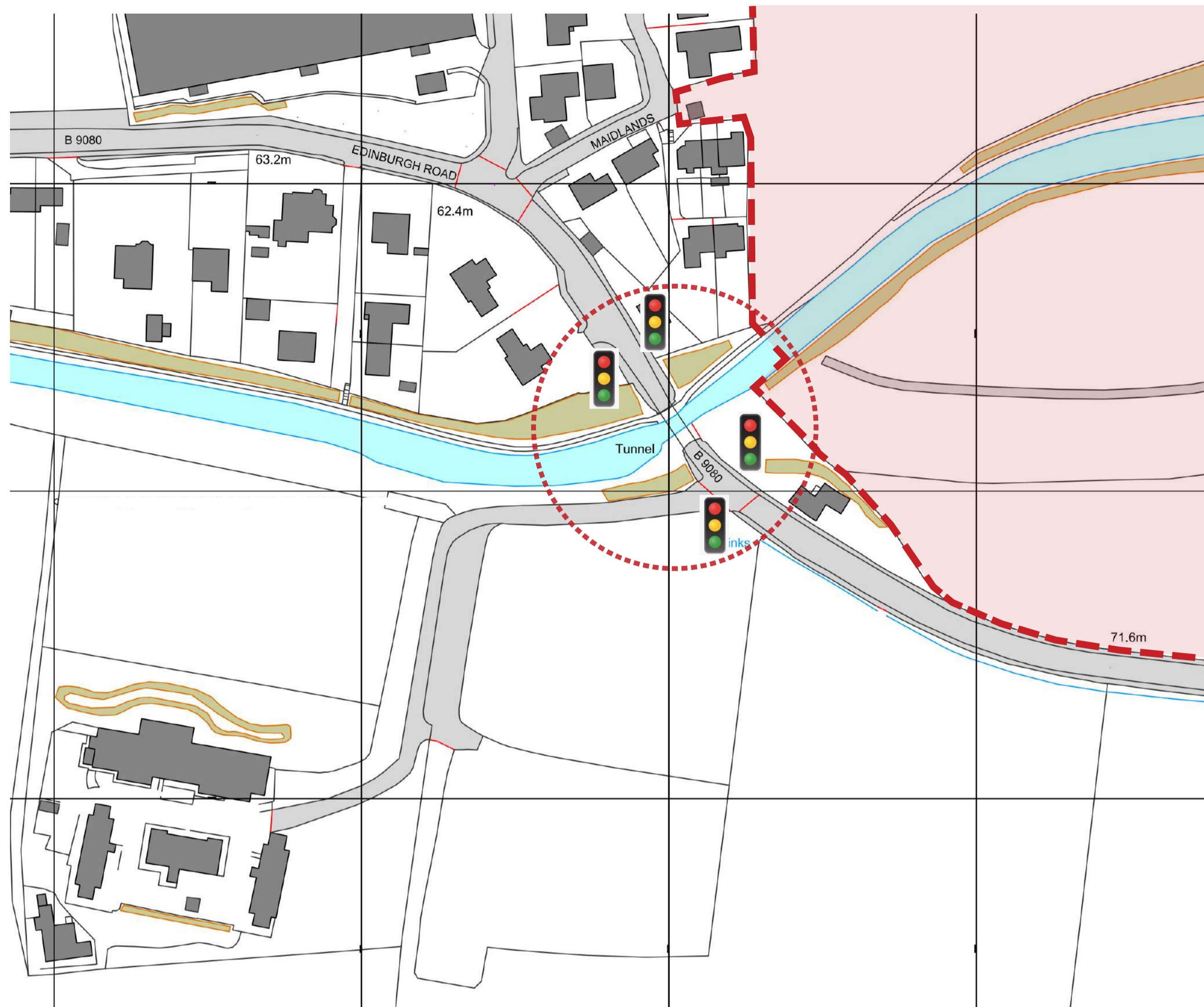
EXISTING TRAFFIC LIGHTS AT BRIDGE ON SOUTHERN SIDE
